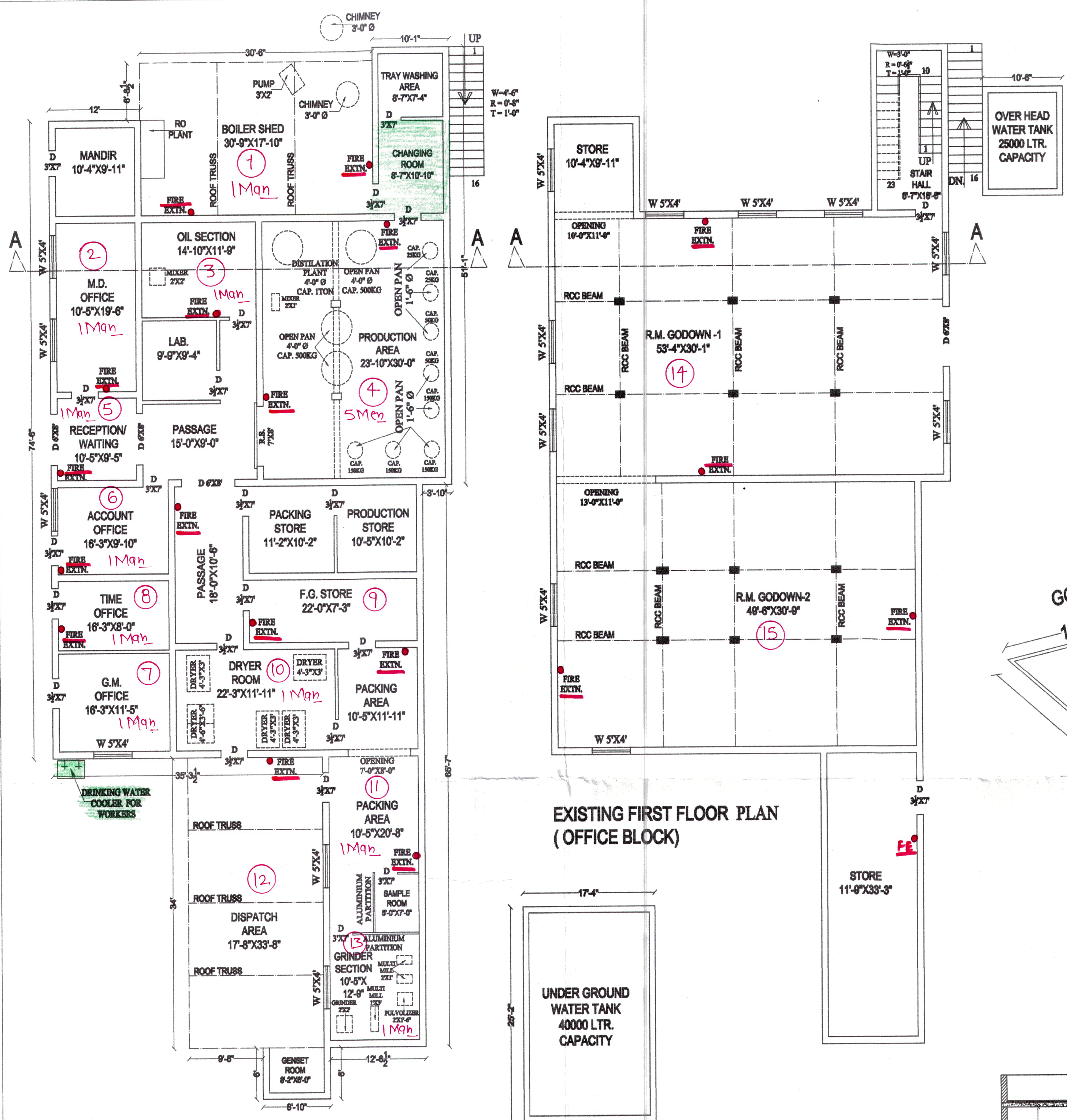
EXISTING GROUND FLOOR PLAN (OFFICE BLOCK)
